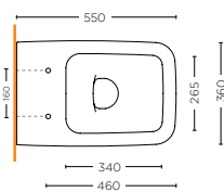
VASO FILO MURO BACK TO WALL WC SCLB.20.F01
